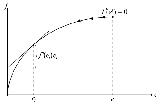
Figure 1. Input Distortion, and Geometry of the Real Population Externality f'(e)e .
