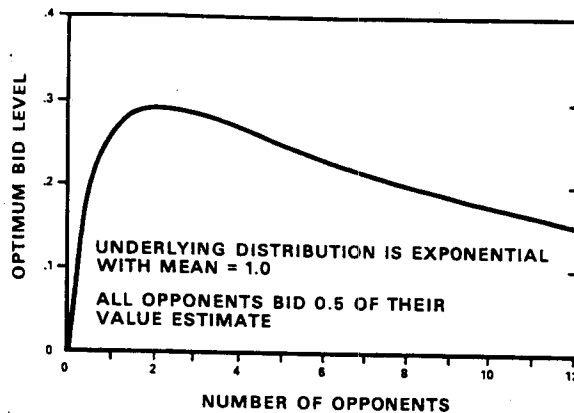
Fig. 5—Optimum bid level vs number of opponents.
