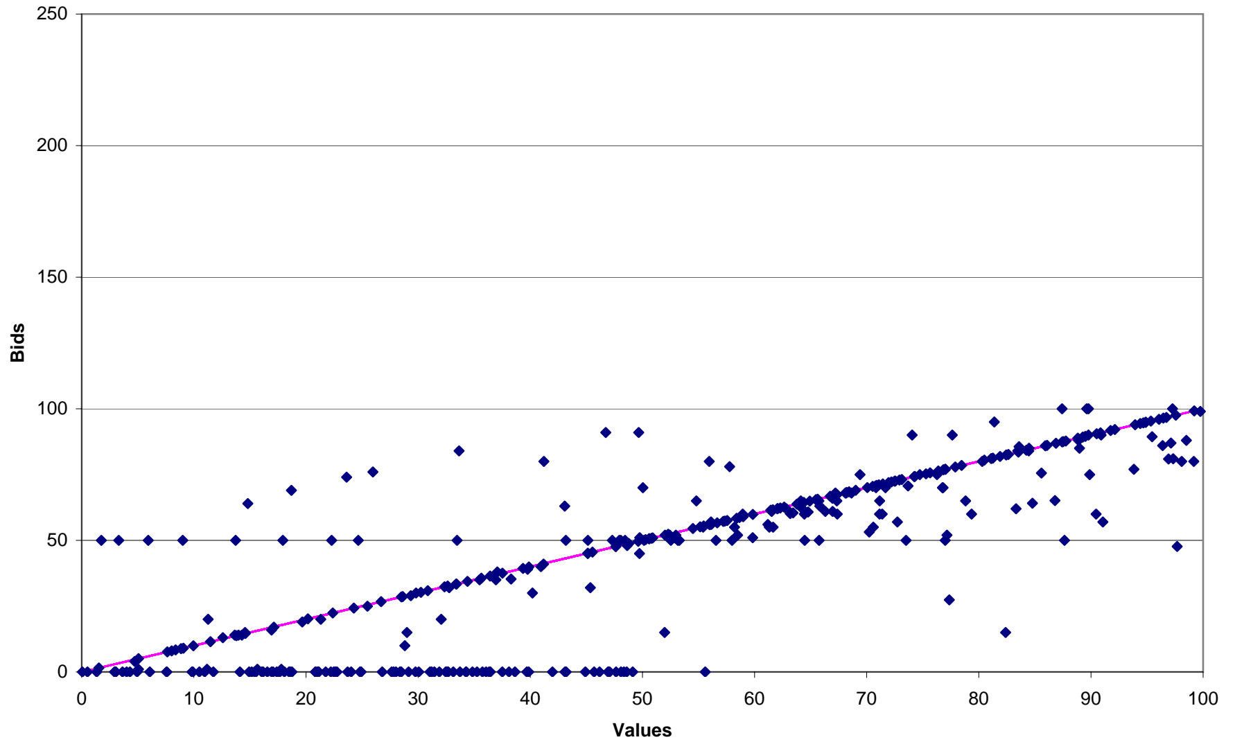
SPA 2-bidder, Reserve = $50, Winter 09
